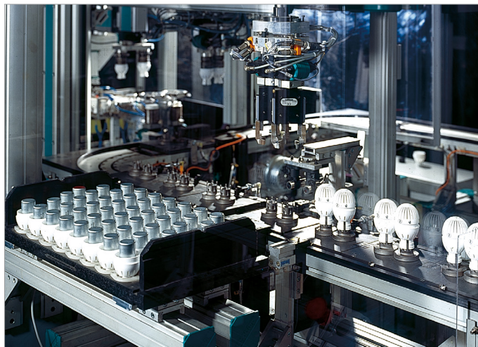
Manufacturing assembly
